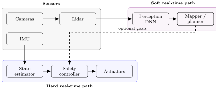
Fig. 3: Dual-path architecture: a hard real-time safety loop (state estimation + safety controller) runs with bounded latency; perception and mapping run asynchronously with watchdog supervision and conservative fallbacks. (Author-created figure.)
