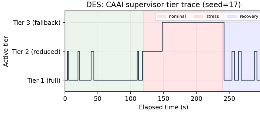
Fig. 9: Discrete-event simulation: CAAI supervisor-selected tier vs. elapsed time for the representative run (seed = 17). Shaded regions mark nominal (0–120 s), stress (120–240 s), and recovery (240–300 s) phases.
