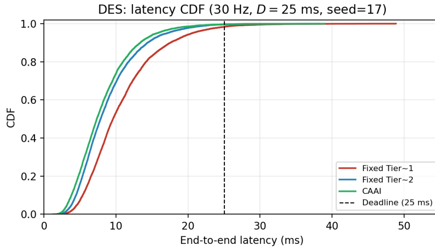
Fig. 7: Discrete-event simulation (Section 6.6): empirical step-CDF of end-to-end latency for fixed Tier 1, fixed Tier 2, and CAAI over the full 300 s run (30 Hz, D = 25 ms, seed = 17). The dashed line marks the deadline.
