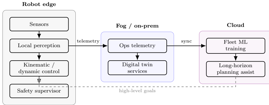
Fig. 5: Typical edge-cloud split: closed-loop safety and actuation remain on-robot; fleet analytics and training reside off-robot with asynchronous interaction. Solid arrows: real-time data flow. Dashed arrow: asynchronous goal delivery from cloud planner to on-robot kinematic controller.
