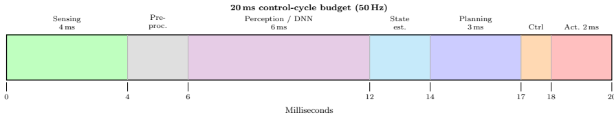
Fig. 1: Visual breakdown of the 20 ms (50 Hz) control-cycle budget. Bar width is proportional to time. The Perception/DNN segment (violet) dominates; Actuation (red) must always be guaranteed. (Author-created figure.)
