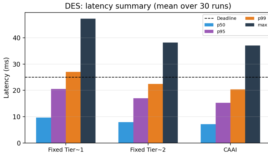
Fig. 8: Discrete-event simulation: mean p50/p95/p99/max latency per condition, averaged over the 30 independent runs reported in Table 13.
